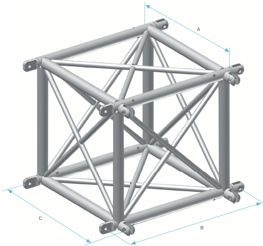
SIZES OF CORNER BLOCKS
