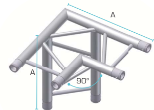
3 WAY HORIZONTAL CORNER 90° LEG DOWN
