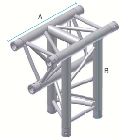
3 WAY VERTICAL TEE APEX DOWN
