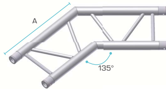
2 WAY HORIZONTAL CORNER 135°
