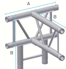
4 WAY VERTICAL TEE PIECE
