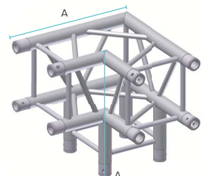
3 WAY CORNER 90°
