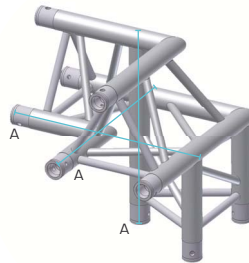
3 WAY CORNER 90° APEX UP RIGHT
