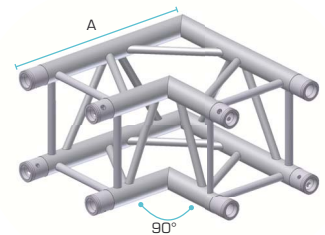
2 WAY CORNER 90°
