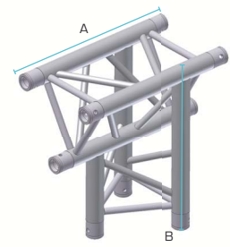
3 WAY VERTICAL TEE PIECE APEX DOWN
