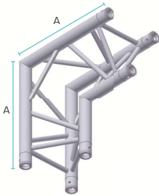
2 WAY CORNER 90° APEX IN
