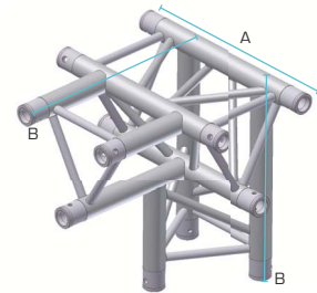
4 WAY TEE PIECE APEX DOWN
