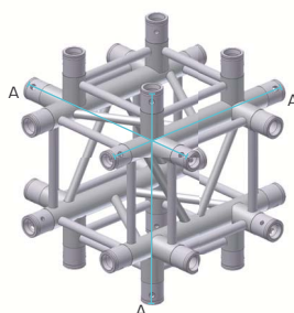
6 WAY CROSS PIECE
