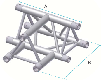
3 WAY VERTICAL TEE PIECE
