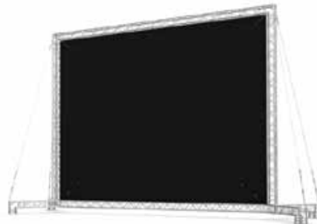
BAN O30 - M290 QUATRO BANNER FRAME width 11500 mm 452.76" length 3100 mm 122.05" height 7300 mm 287.40"
