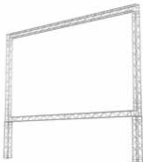
BAN O40 - M290 QUATRO BANNER FRAME (FOLDABLE) width 9000 mm 354.33" length 300 mm 11.81" height 7000 mm 275.59"
